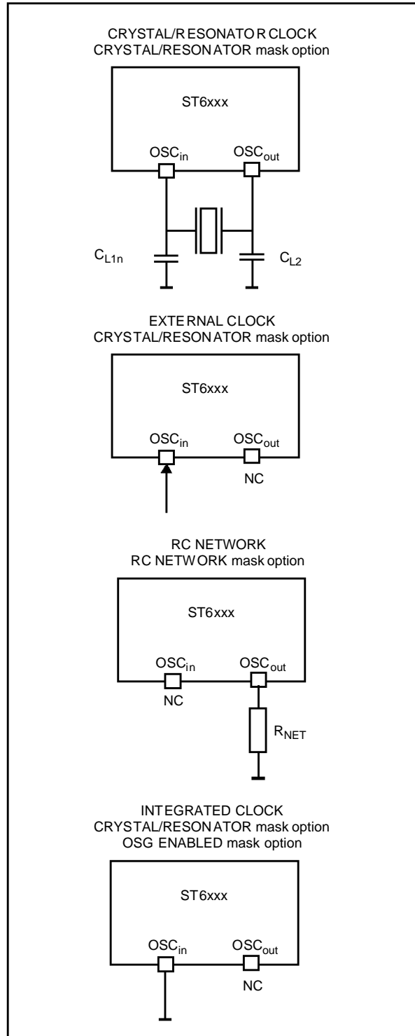
Figure 10. Oscillator Configurations
