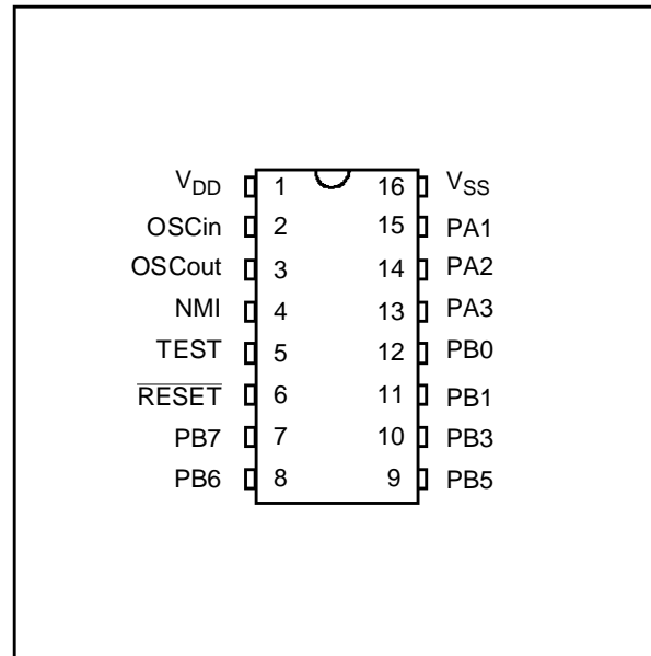
Figure 4. ST6203B Pin Configuration
