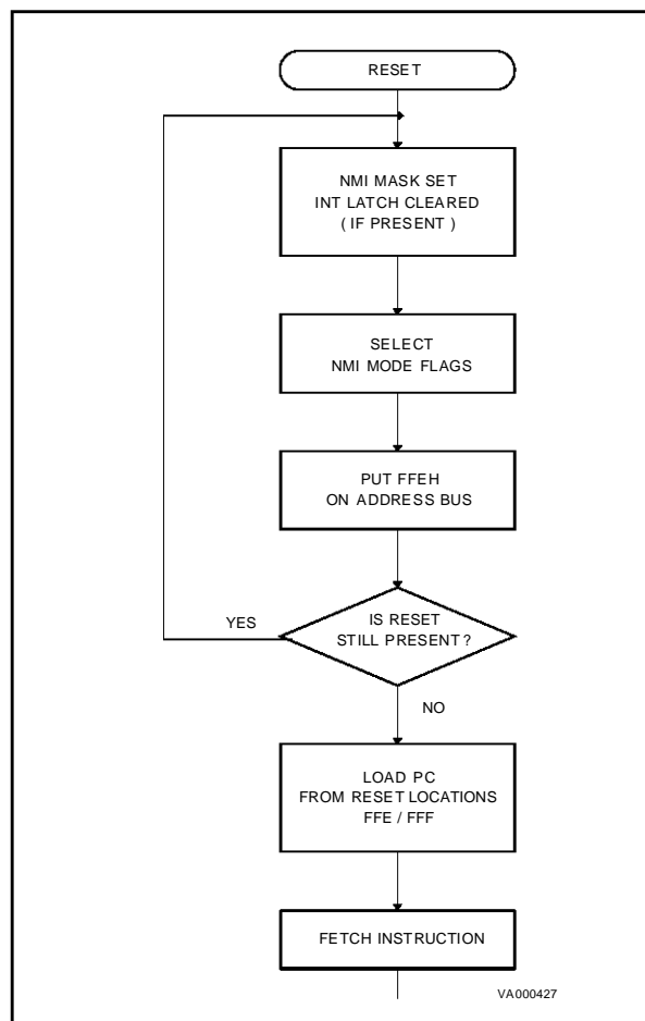
Figure 15. Reset and Interrupt Processing
